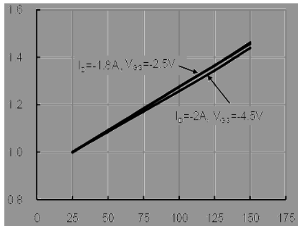
Figure 4 Drain-Source On-Resistance
